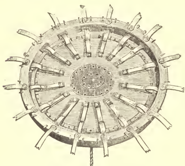
Balloon Valve Invented by M. Giffard.
